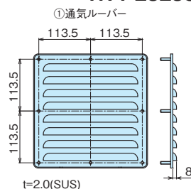
HVT-2525S-G
